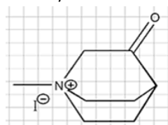
1-methyl-quinuclidine-3-on-iodide
