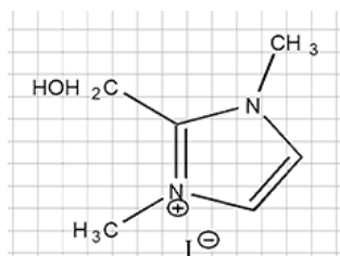
1,3-dimethyl-2-hydroxyethyl-imidazolyl-iodide
